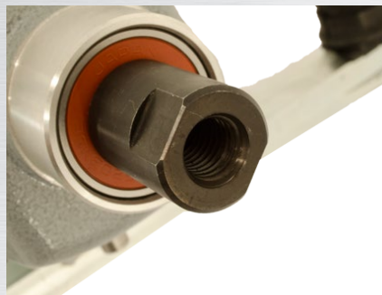
Tool connection thread M14 internal
